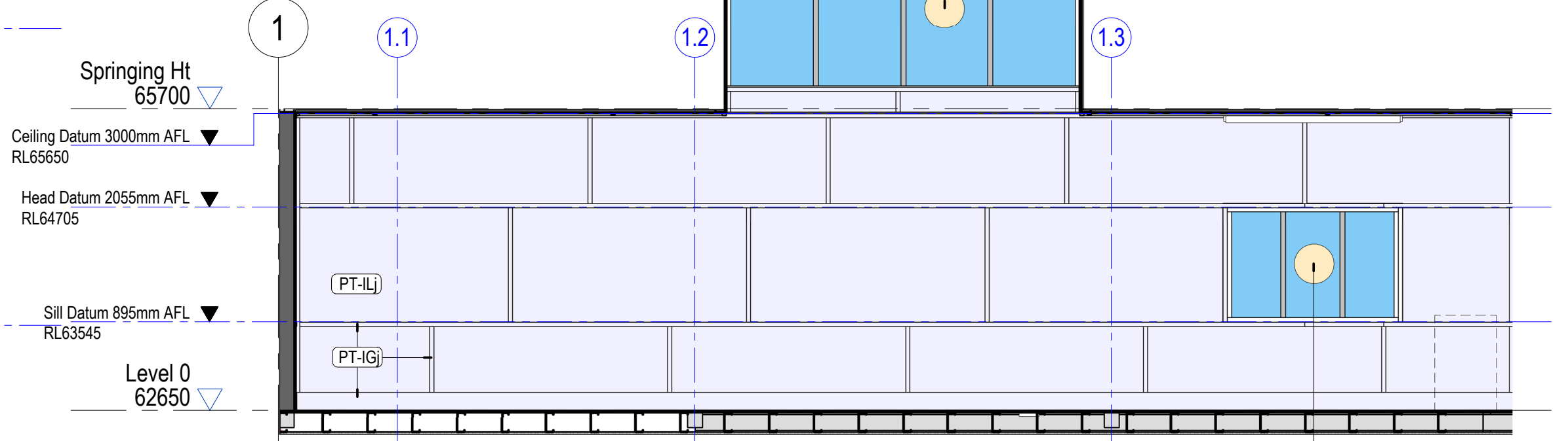
0.35 - Workspace (east) - East Elevation 1:50
